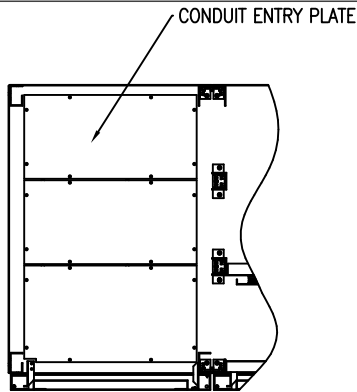
BOTTOM CABLE ENTRY CROSS SECTION A-A
