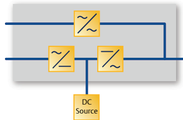
Distributed Bypass (1+N) Parallel up to 6 modules
