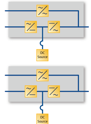
Dual Bus 2N Tier 2-4
