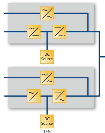
Distributed Bypass (1+N) Parallel up to 6 modules
